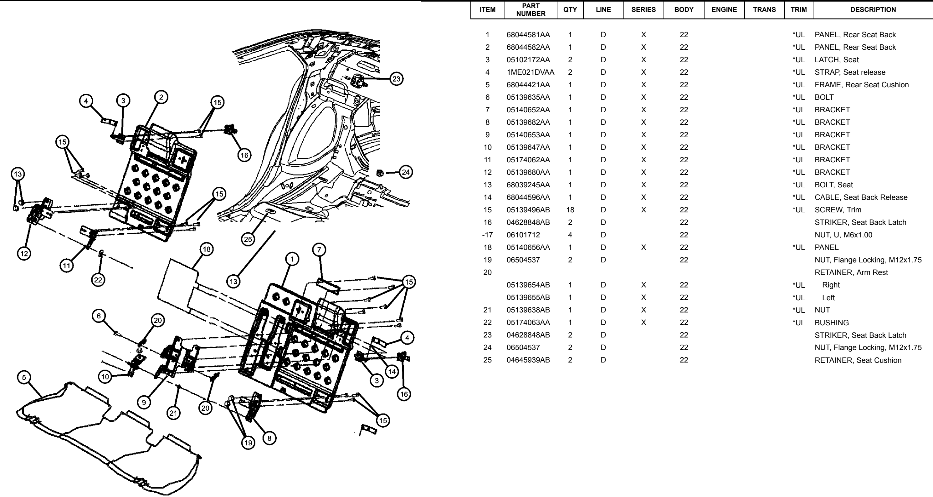
Second Row - Split Seats Figure 50-1030
