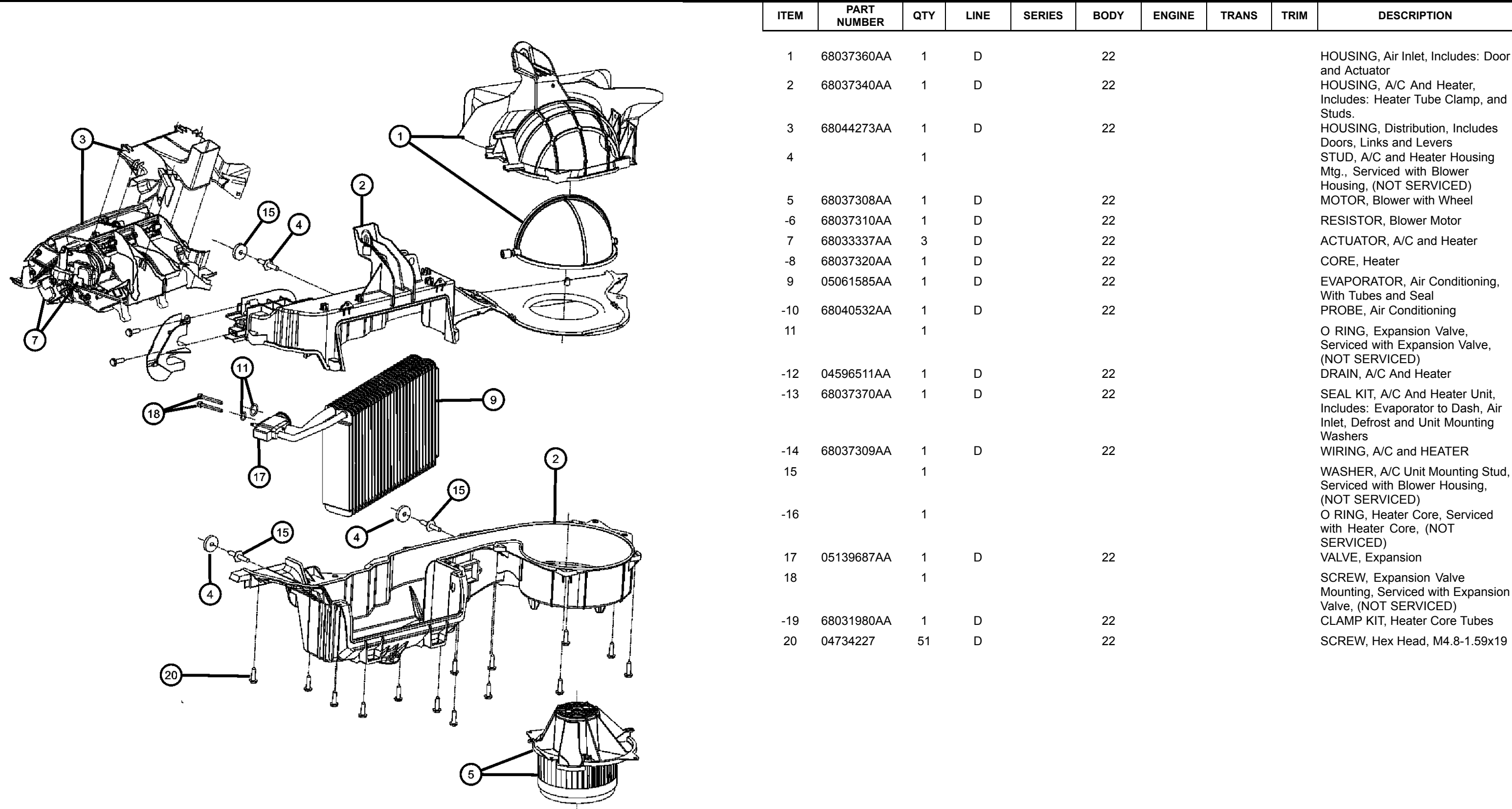
A/C and Heater Unit Figure 24-120
